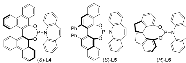
Scheme 1. Phosphoramidite–alkene ligand screening.
